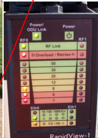
Link performance, signal display level 8 @ pointing to the stone building to receive in NO Line Of Sight beamed at reverse and only by reflexion
